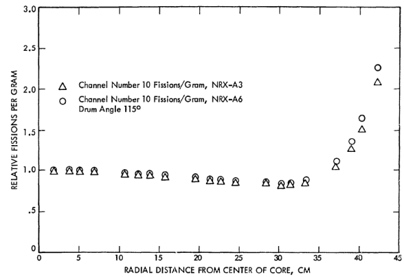
Figure 4-8. Comparison of the NRX-A3 and NRX-A6 Predicted Power Distributions through Traverse 008 to J5L, Fission Per Gram
