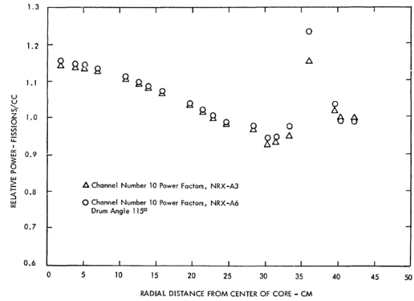
Figure 4-6. Comparison of the NRX-A3 and NRX-A6 Predicted Power Distributions through Traverse 008 to J5L, Fissions/cc
