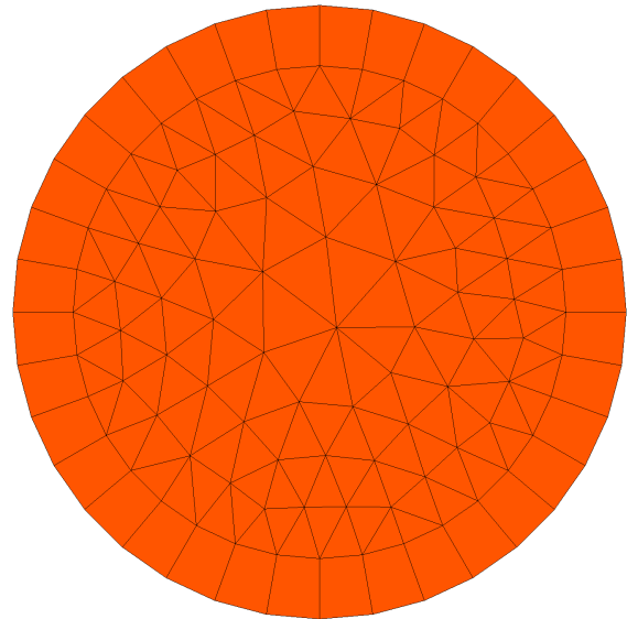
(d) Iteration 4.0: Adequate y^+ margin along the full pipe length with smooth transition to the bulk and angular aperiodicity; final mesh used
