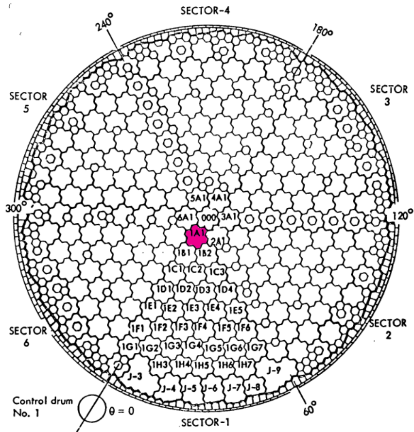
Figure B.4: NRX-A6 core map with thermocoupled hot cluster 1A1 in magenta
