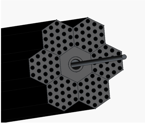
(a) Fuel cluster cold end without the hardware shown in fig. 4.3
