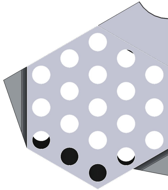
(b) Partial implementation of a cluster a single fuel element and central unfueled element as well as support block cut into corresponding 1/6th sections
