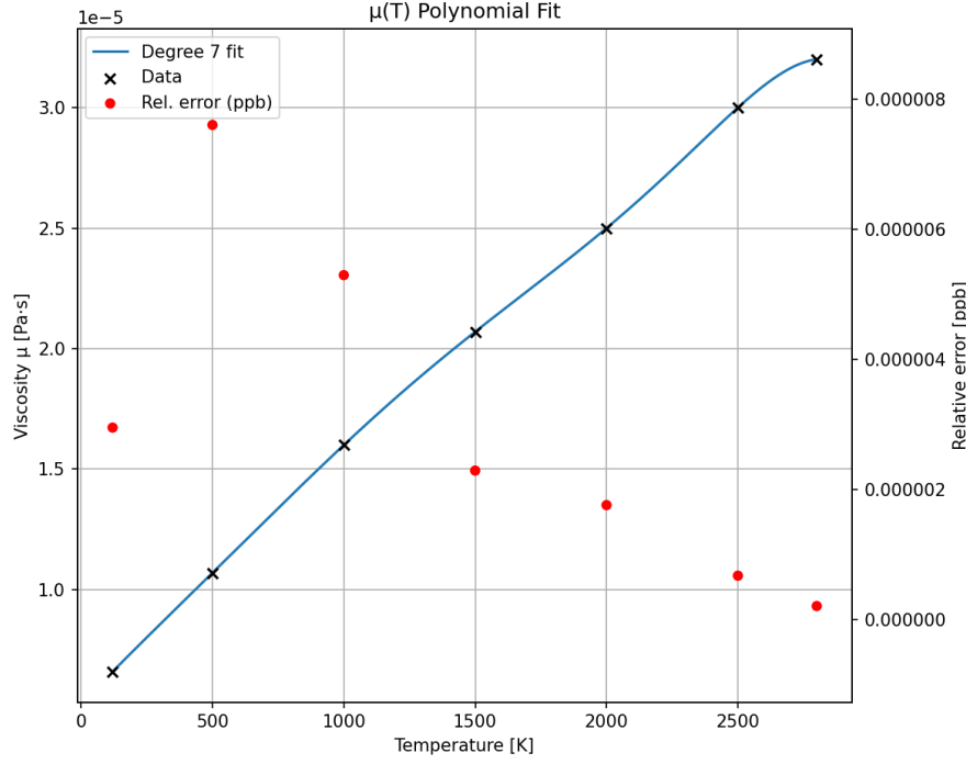
Figure 5.9: Seventh-degree polynomial fit for hydrogen dynamic viscosity as a function of temperature at pressures between 4 & 5 MPa, including relative error compared to data points
