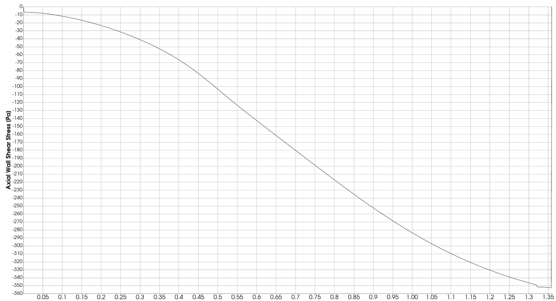
Figure 6.7: Axial distribution of wall shear stress on the fluid
