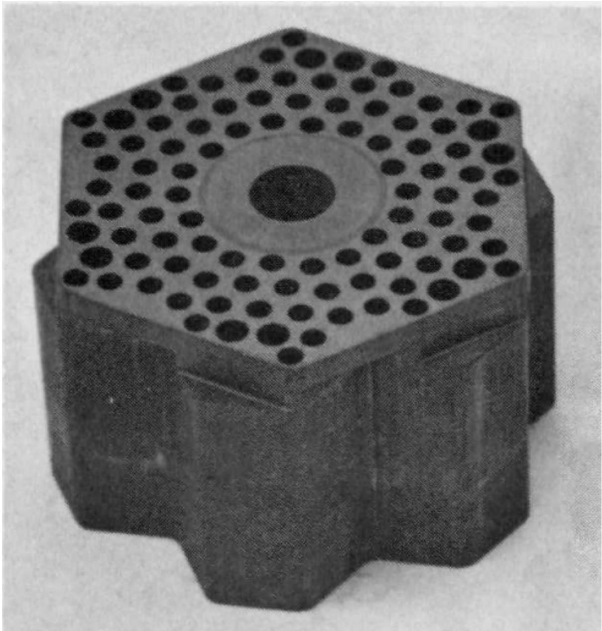
(a) Same support block as in fig. C.5 but with 19.05 mm (0.75in) machined away from TME-1373 fig. 3-2
