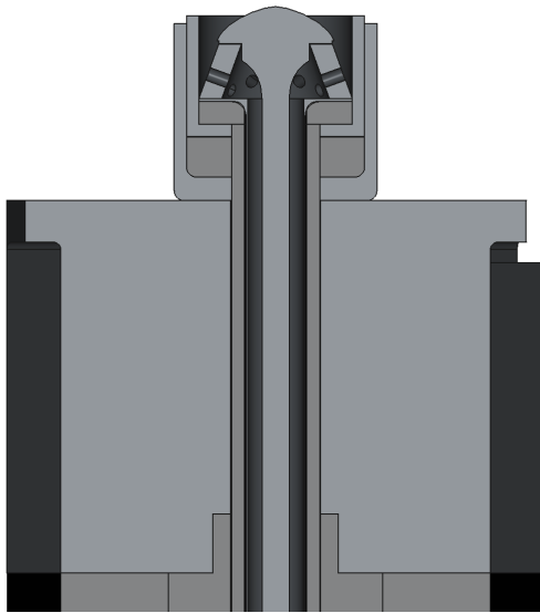
(c) Cutaway view of the cluster hot end
