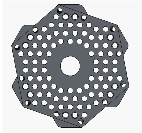
(b) Support block hot-end view in FreeCAD.
