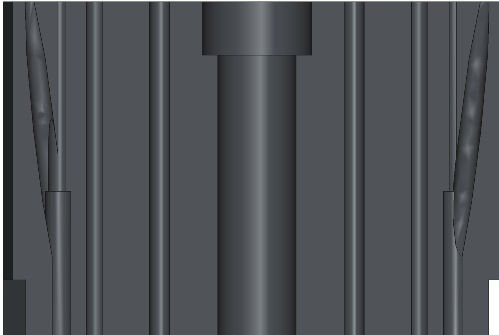
(c) Cut into Support Block showing the unification of channels
