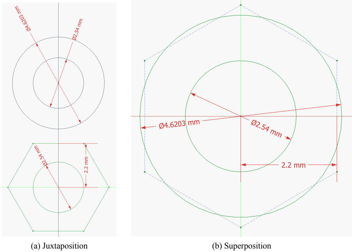
Figure 5.3: Comparison of the hexagonal coolant-channel cross section and its equivalent circular representation in FreeCAD.
