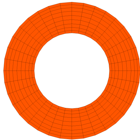
(d) Iteration 4.0: Custom cross-section with stretch factor 1.18 from both edges, yielding optimal accuracy–efficiency trade-off; (final configuration used)
