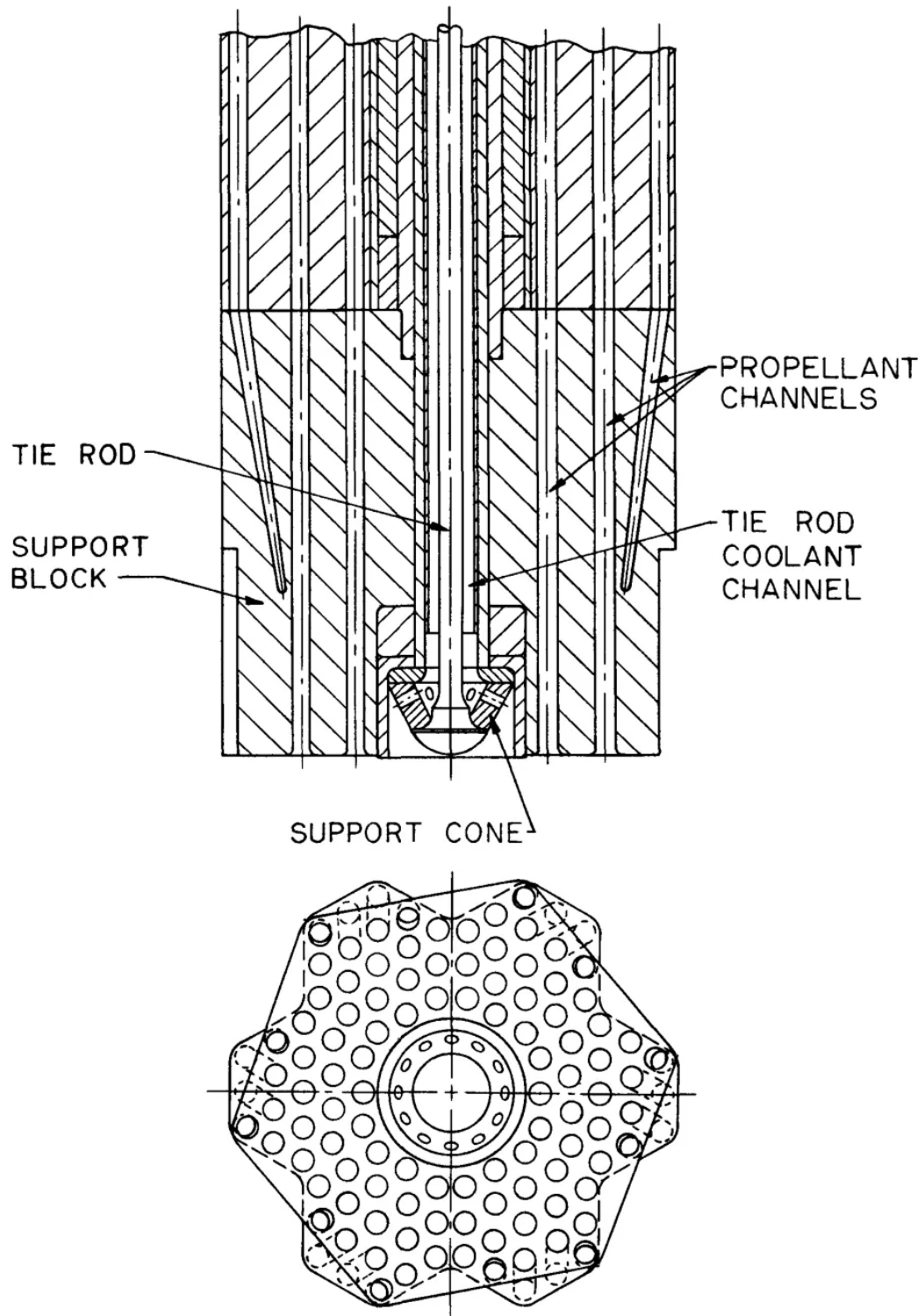
FIGURE 1 SUPPORT BLOCK END OF SEVEN-ELEMENT CLUSTER
