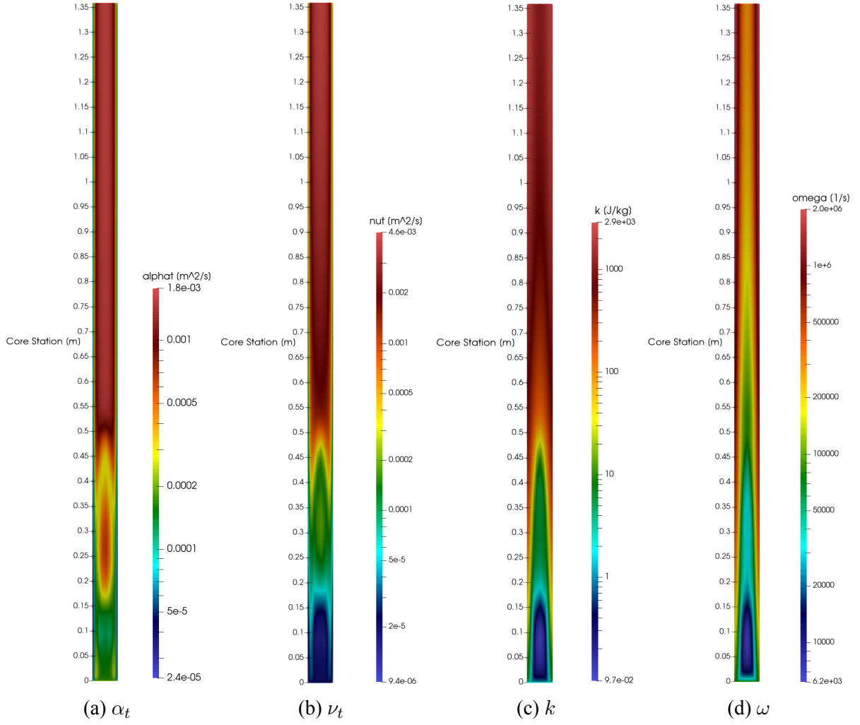
Figure 6.11: Color maps of all turbulence fields for the kOmegaSST-model (aspect ratio scaled down \times 20 for visibility)
