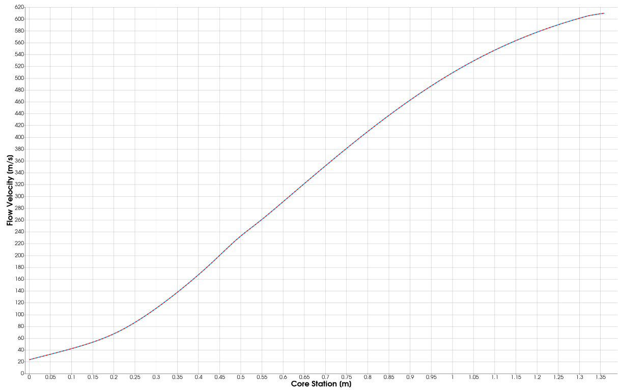
Figure 6.6: Legend: blue solid: |\vec{U}| in propellant bulk center ( r = 0 mm); red dashed: U_z propellant–solid interface ( r = 0 mm);
