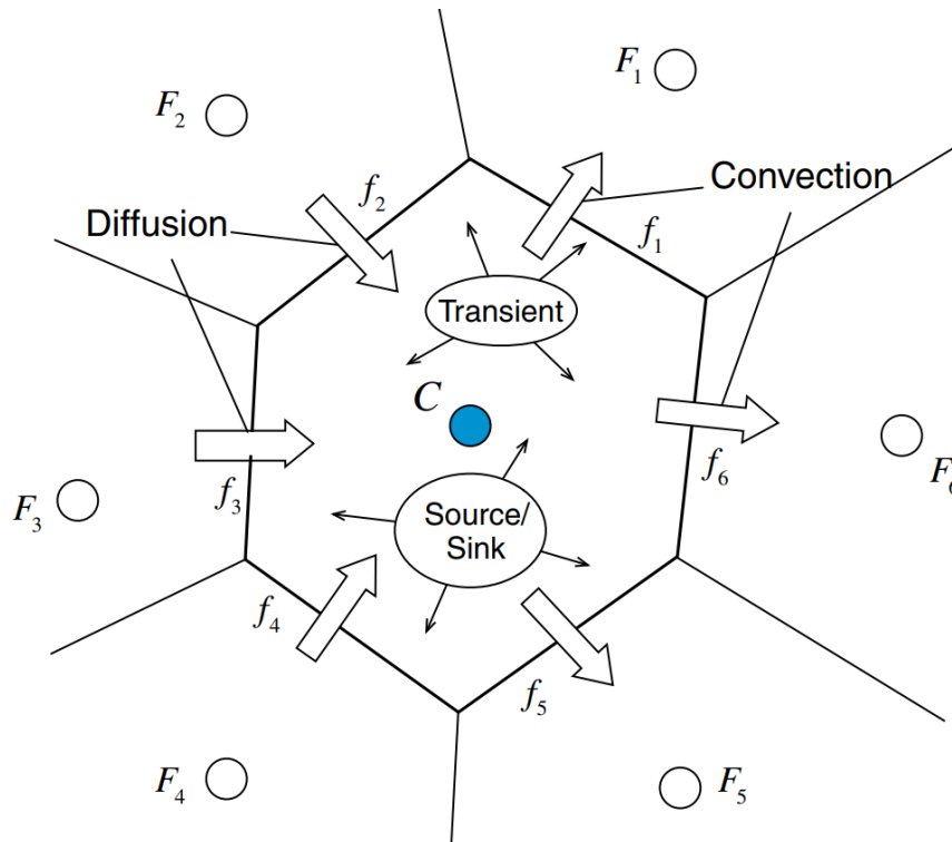
Figure 3.2: Example schematic of a control volume C with its faces ( f_1 to f_N ) neighbouring finite volume cells (with centers F_1 to F_N ) - Source: [22, fig. 16.1]
