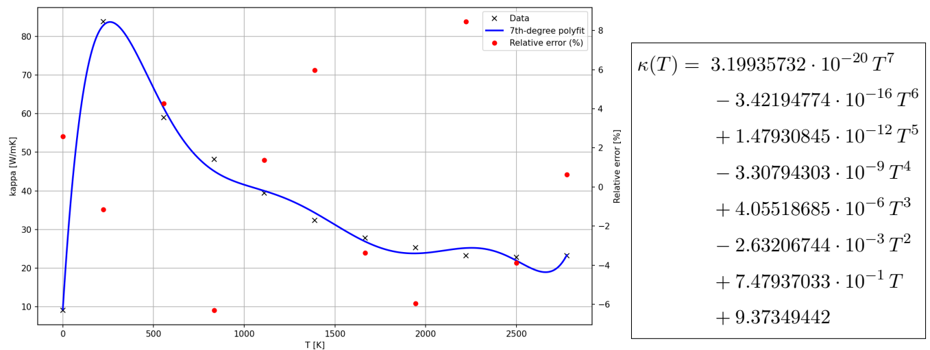
Figure 5.6: Polynomial fit for fuel element thermal conductivity
