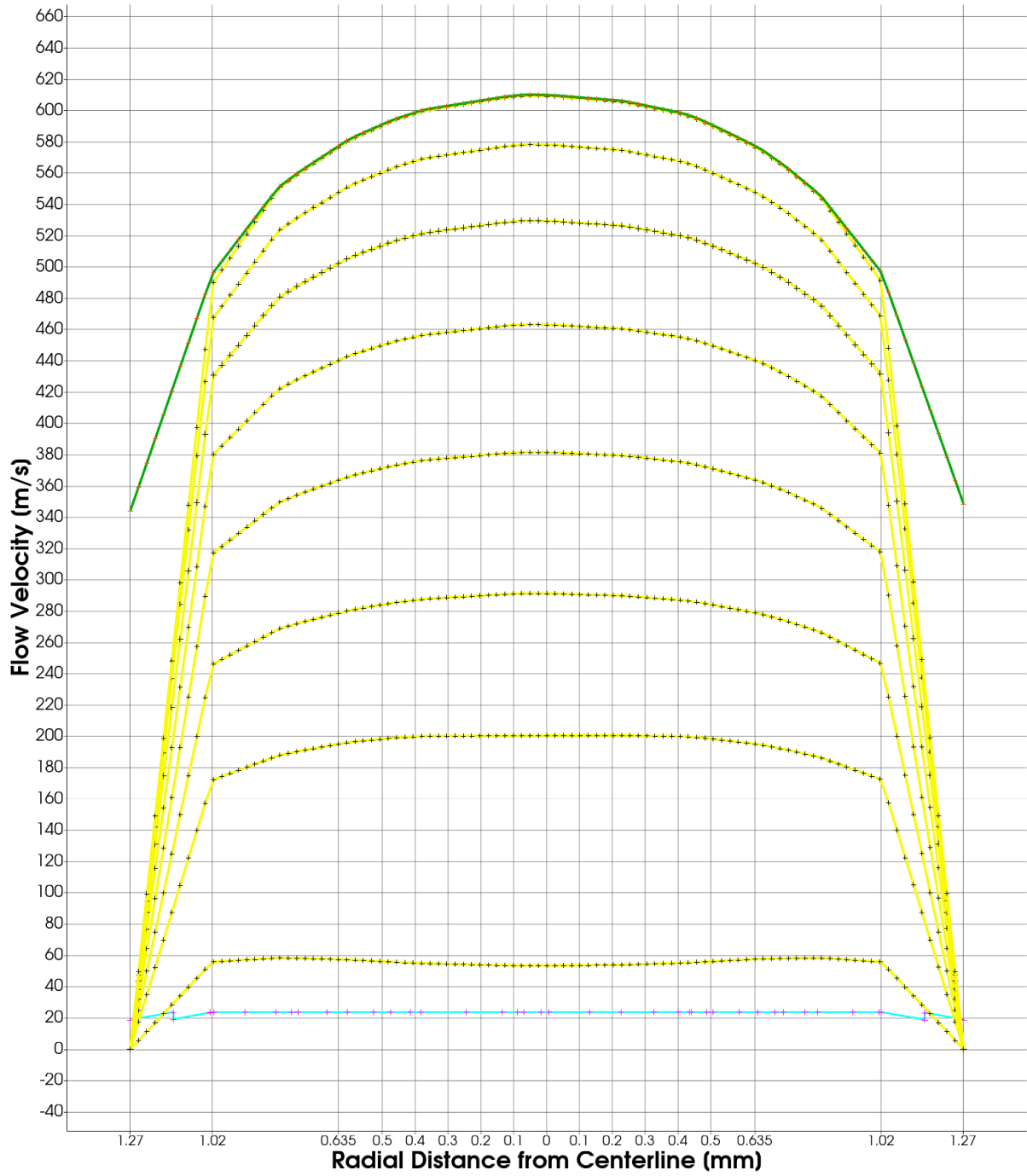
Figure 6.8: Radial Velocity Profiles - Legend:
