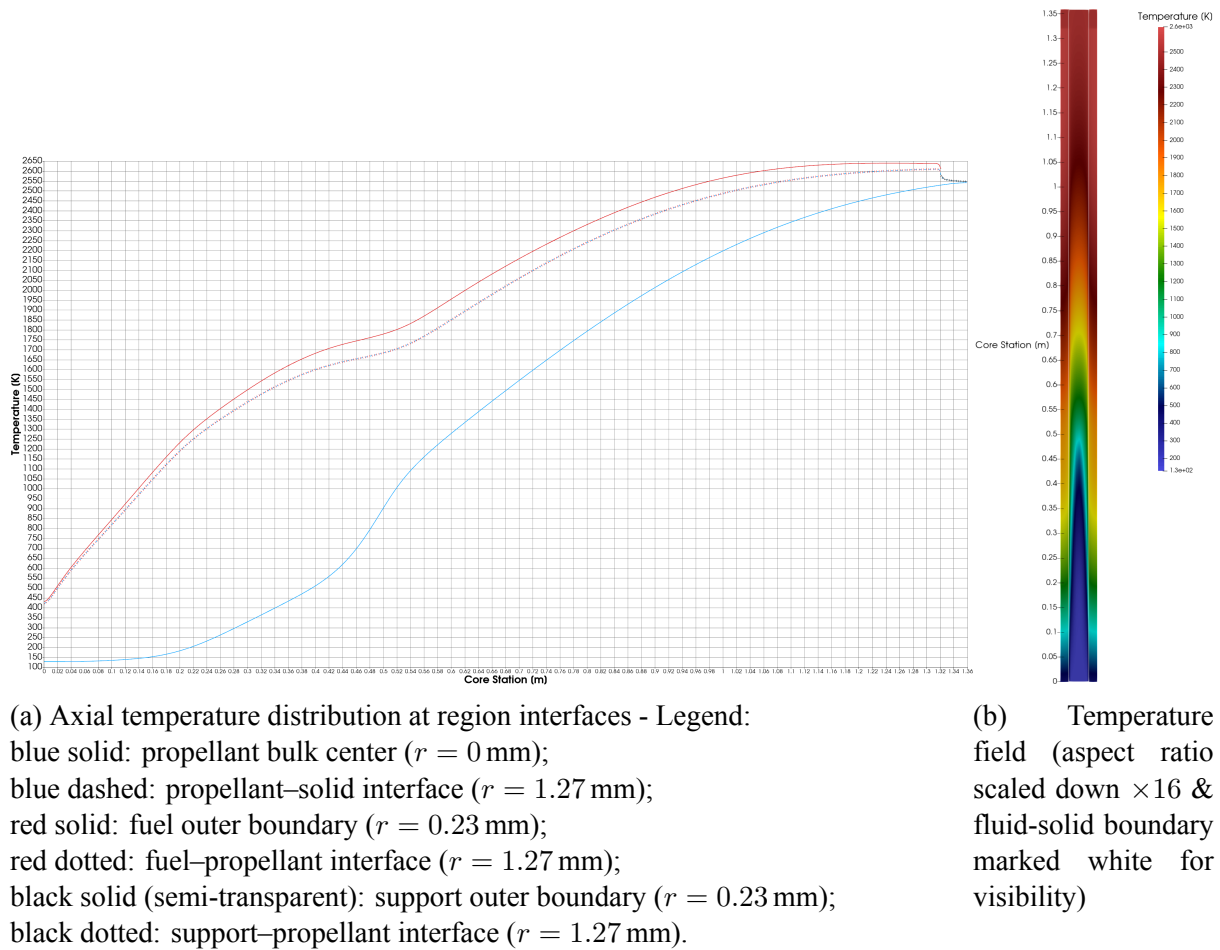
Figure 6.1: Axial temperature profiles and corresponding temperature field color map through centerline cut.
