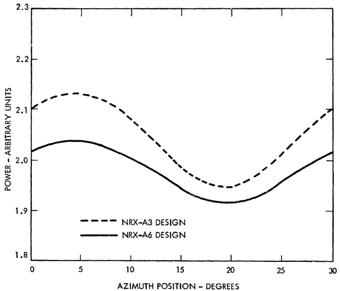
Figure 4-9. Comparison of the NRX-A3 and NRX-A6 Power Scalloping at the Periphery of the Cone, Exterminator Predictions
