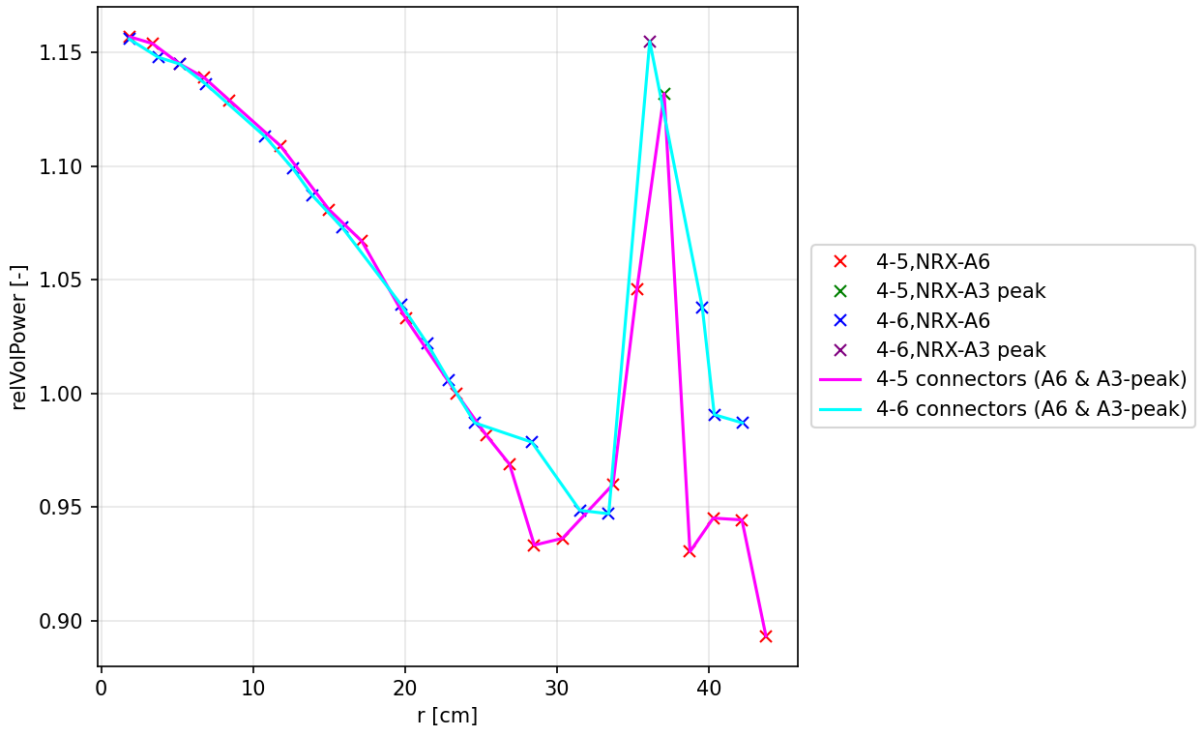
Figure 5.13: Relative radial power distributions predicted for two different azimuths within NRX-A6 supplemented with respective NRX-A3 values for peripheral peak estimation and linear connectors added
