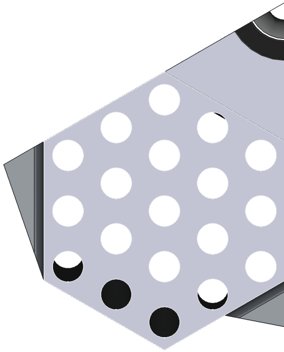
(a) Partial implementation of a cluster a single fuel element and all parts coaxial centerpoint of the unfueled element cut into corresponding 1/6th sections
