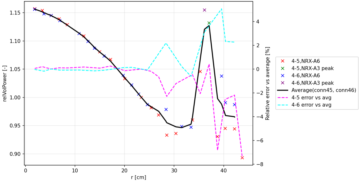
Figure 5.14: Black line shows arithmetic mean of both linear connector graphs; red, green, blue and purple show original data points; cyan and magenta dotted lines show relative error for the averaging process compared to original connector graphs in fig. 5.13
