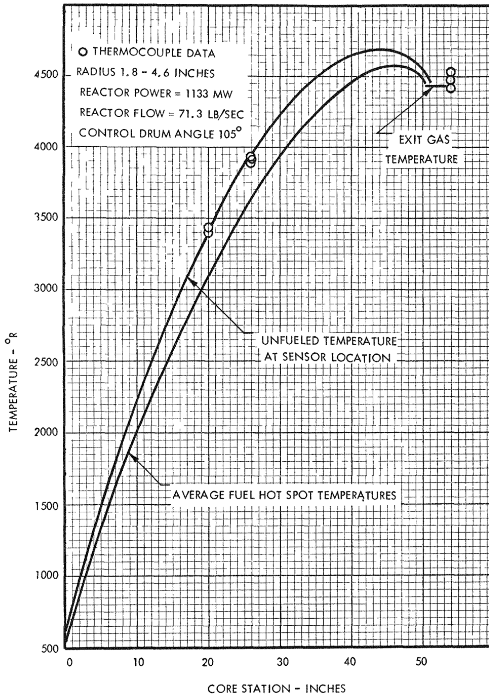
Figure 6. (U) Core Central Region, Axial Temperature Distributions During Power Hold
