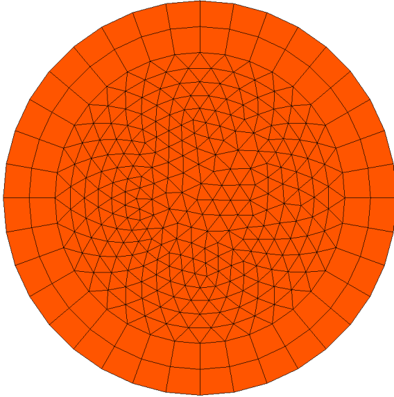
(c) Iteration 3.0: Insufficient y^+ margin to ensure wall-function validity across entire wall length; resolution contrast between wall and bulk is excessive.
