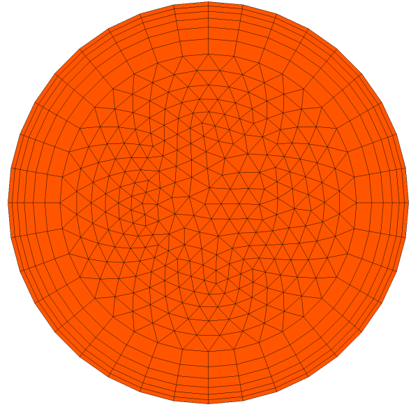
(b) Iteration 2.0: Attempt to fully resolve the boundary layer with y^+ \approx 1
