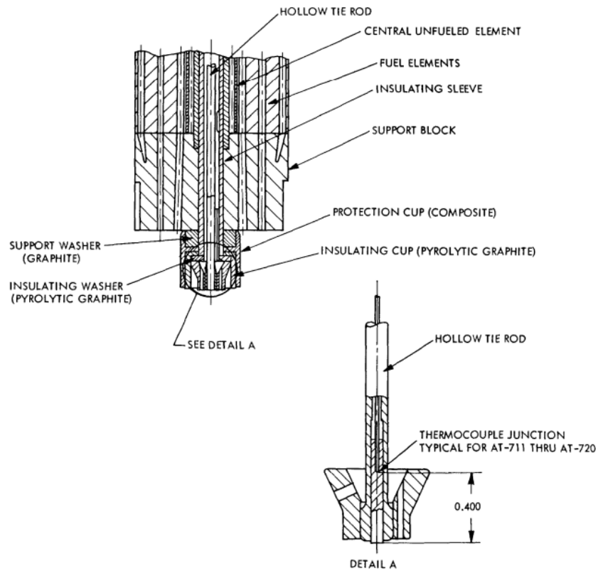
(a) Support block hardware detail used in NRX-A6 from the Transducer Evaluation Report; note that the tie rod is atypical due to the presence of a thermocouple.
