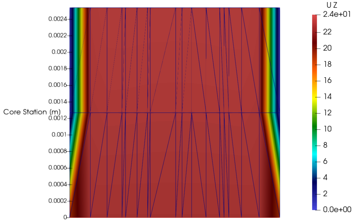
(a) Development of the velocity boundary layer over the first 2 cells at the inlet
