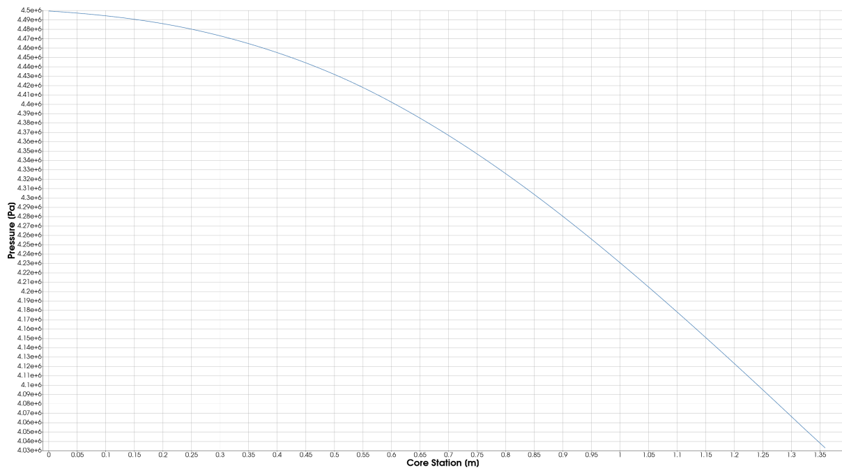
Figure 6.4: Axial pressure distribution in the channel - No color map is presented for pressure because the field is radially isobaric.
