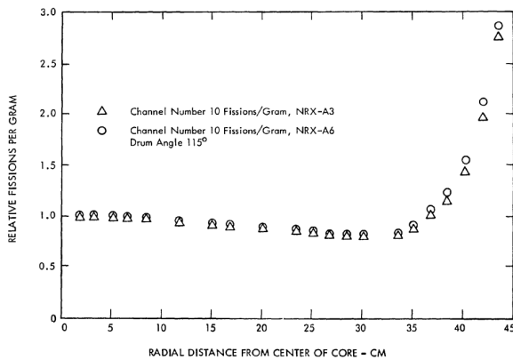
Figure 4-7. Comparison of the NRX-A3 and NRX-A6 Predicted Power Distributions through Traverse 008 to J4M, Fissions Per Gram
