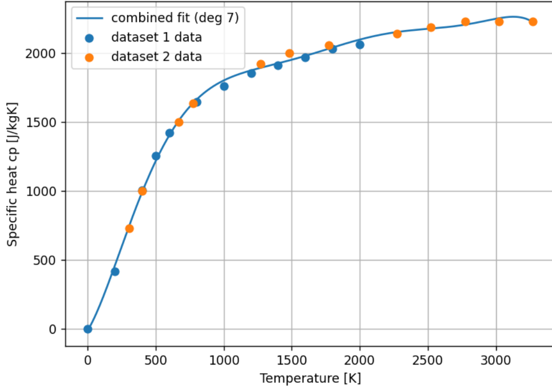
Figure 5.7: Specific Heat of Graphite
