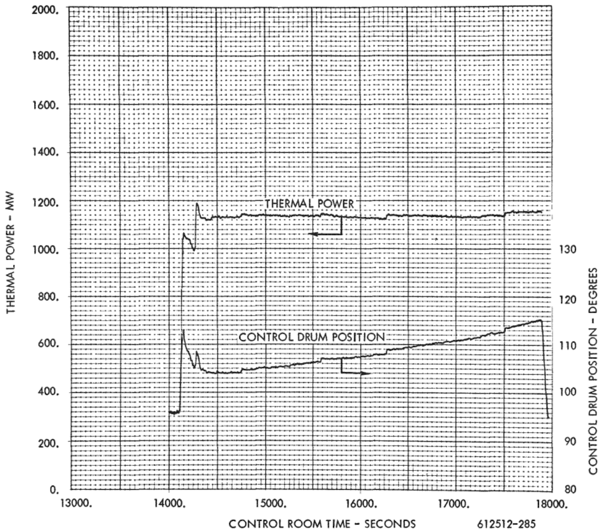
Figure B.3: NRX-A6 actual total reactor power over time
