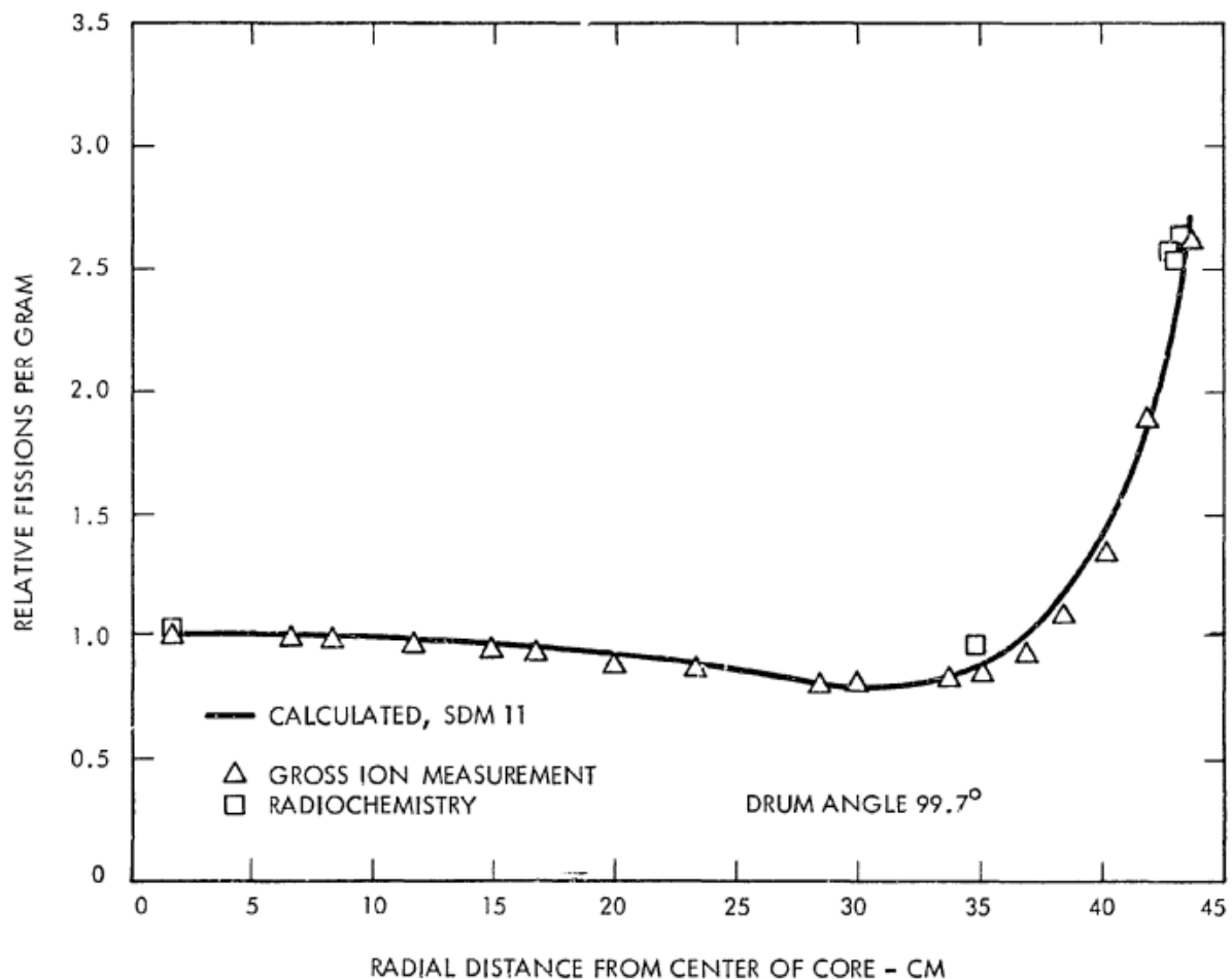
Figure 4-4. Comparison of the NRX-A2 Measured and Predicted Power Distributions through Traverse to J4M, Fissions Per Gram
