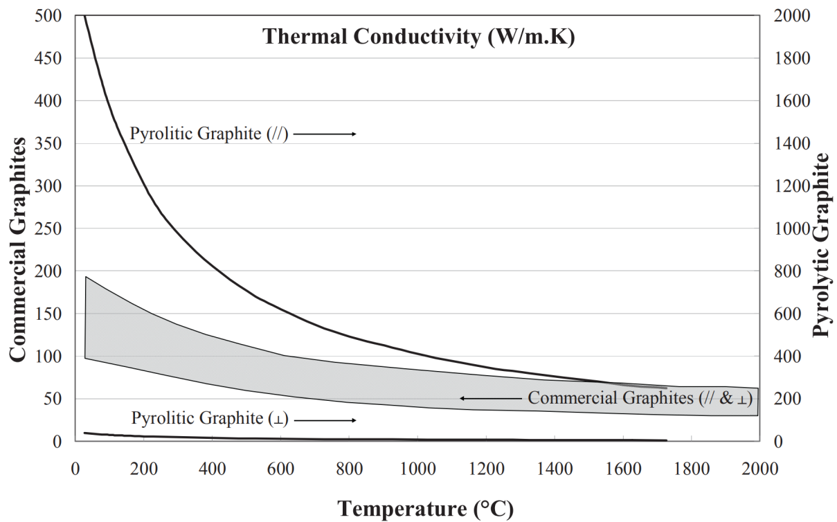
Figure 7.2: Thermal conductivity of pyrolytic and other forms of graphite - Source [34, fig. 6]
