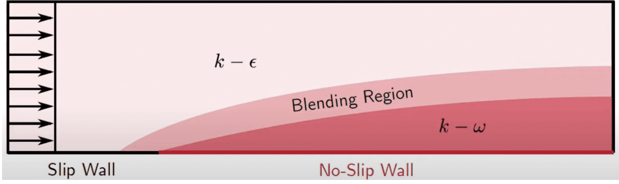
Figure 3.3: kOmegaSST model blending k - \omega and k - \epsilon - Source: SimScale
