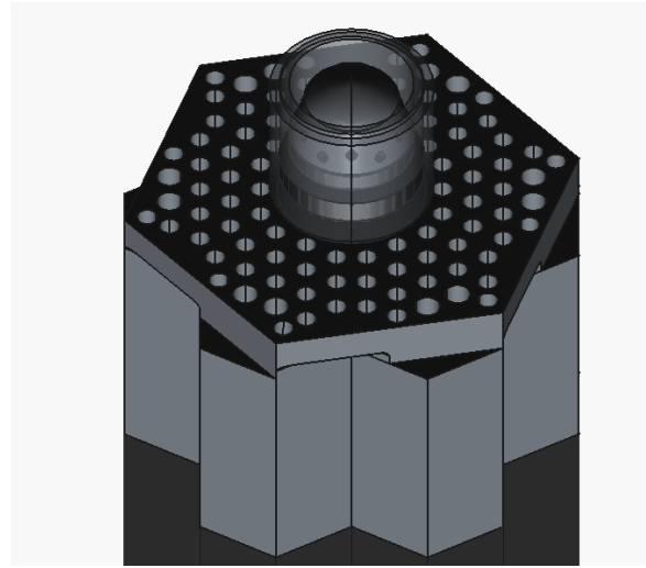
(b) NRX-A fuel cluster hot end with “skirtless” support block and hardware (partially transparent) thermohydraulically equivalent to NRX-A6
