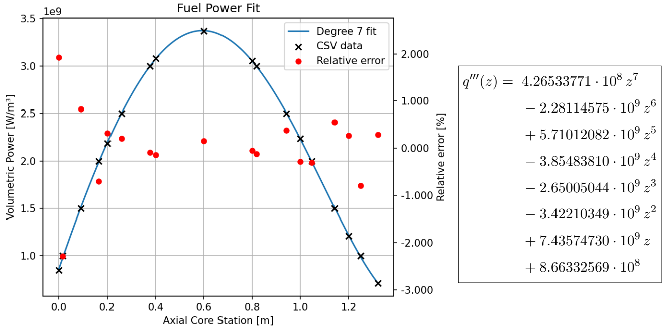
Figure 5.12: Seventh-degree polynomial representation of axial distribution of volumetric power based on points taken from Wang’s & Kotlyar’s graph
