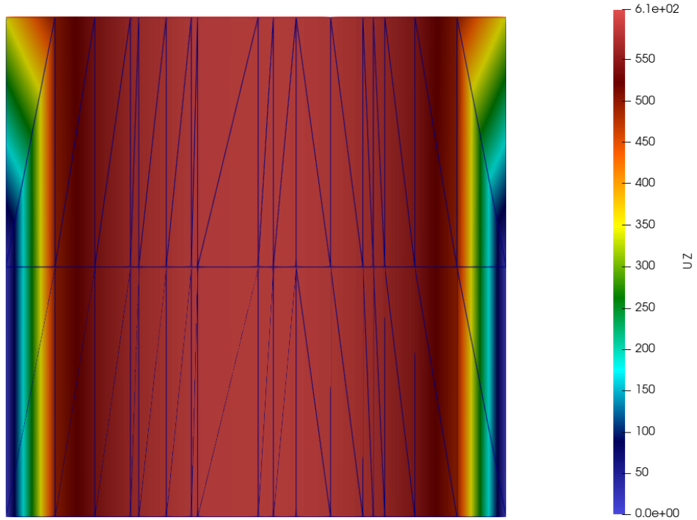
(b) Dissolution of the velocity boundary layer over the last 2 cells at the outlet
