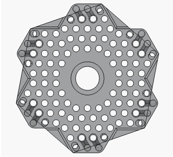
(a) Transparent view from the side interfacing with core elements.
