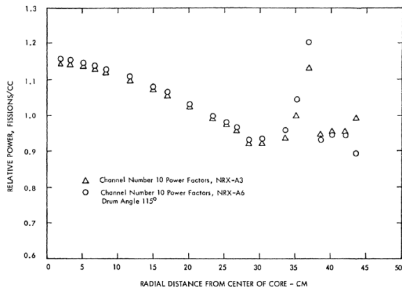
Figure 4-5. Comparison of the NRX-A3 and NRX-A6 Predicted Power Distributions through Traverse 008 to J4M, Fissions/cc
