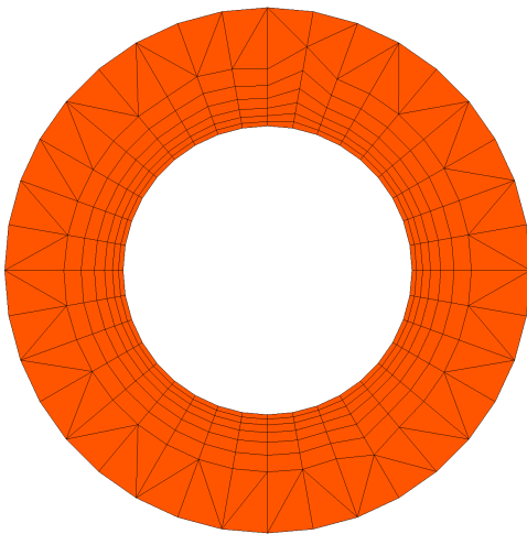
(c) Iteration 3.0 using NETGEN algorithm: breakdown of zeroGradient boundary condition at the outer edge
