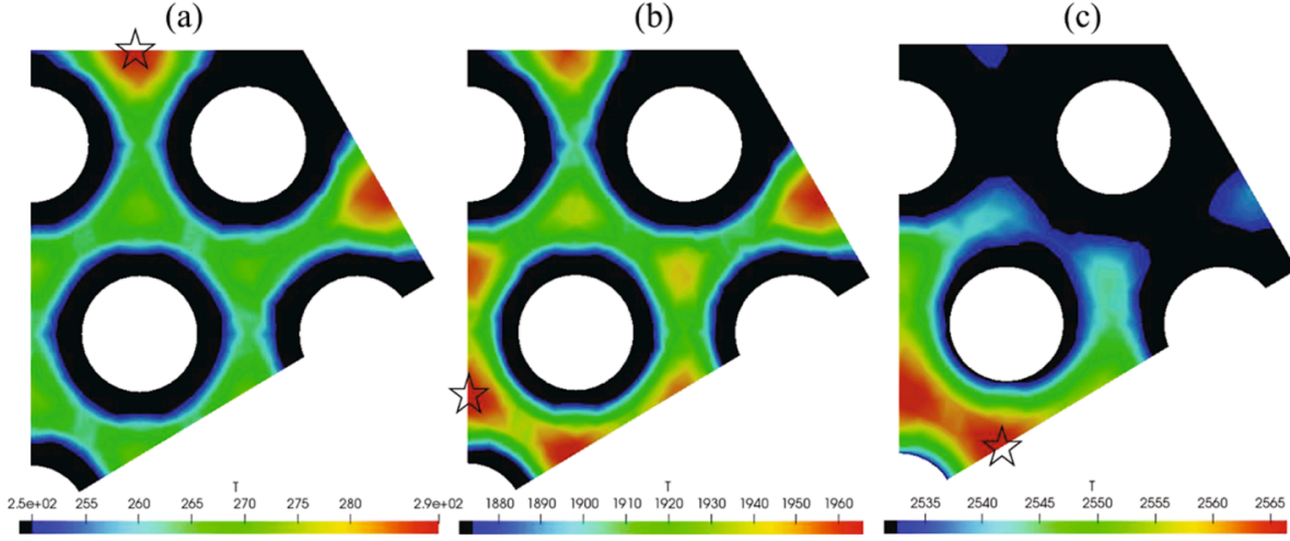
Figure 5.2: Cross-sectional temperature variability inside Fuel Element
