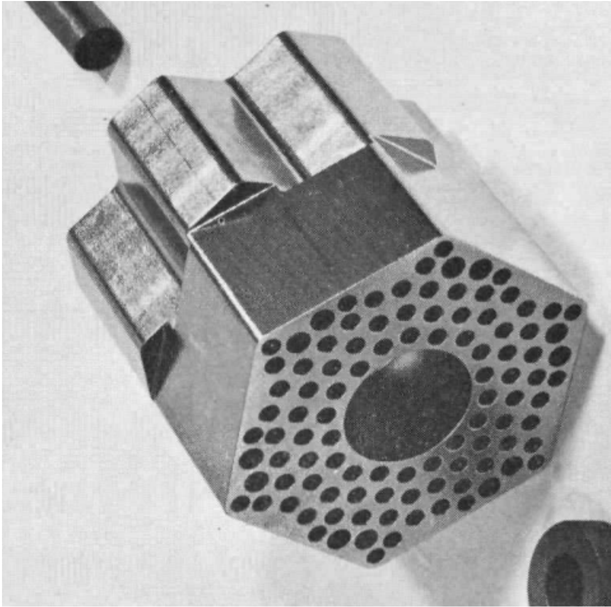
Figure C.5: NRX-A5 support block source WANL-TME-557 Fig. B.4
