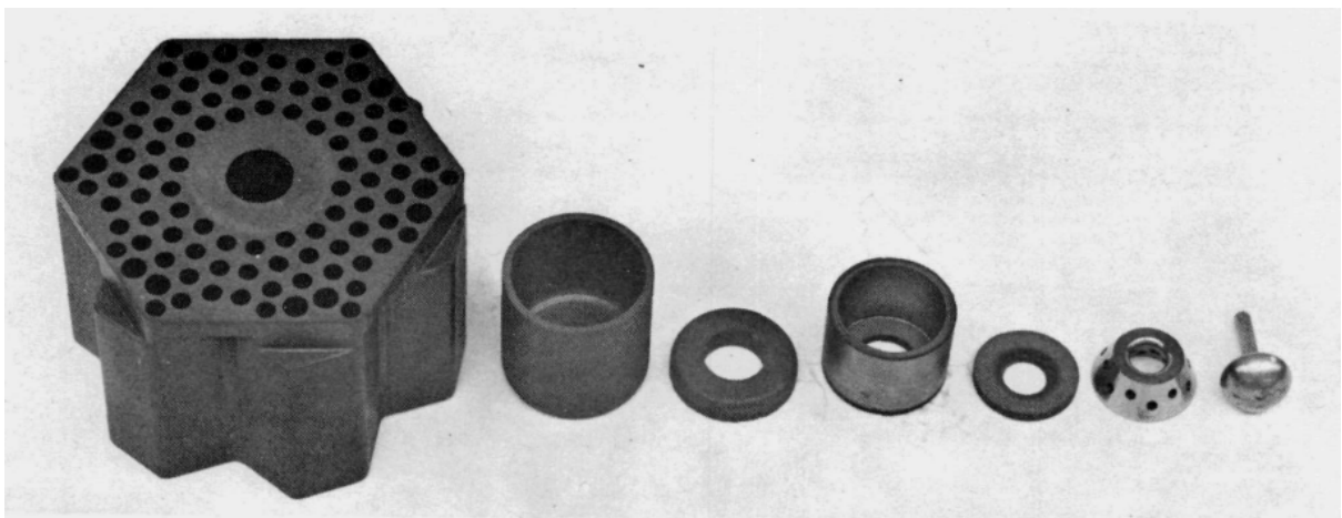
(b) Support block designated as being for NRX-A6 in WANL-TME-1373 fig. 5-1
