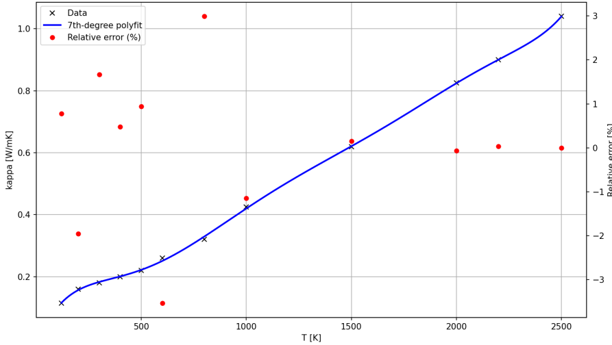
Figure 5.10: Seventh-degree polynomial fit for hydrogen thermal conductivity as a function of temperature at pressures between 4 & 5 MPa, including relative error compared to data points
