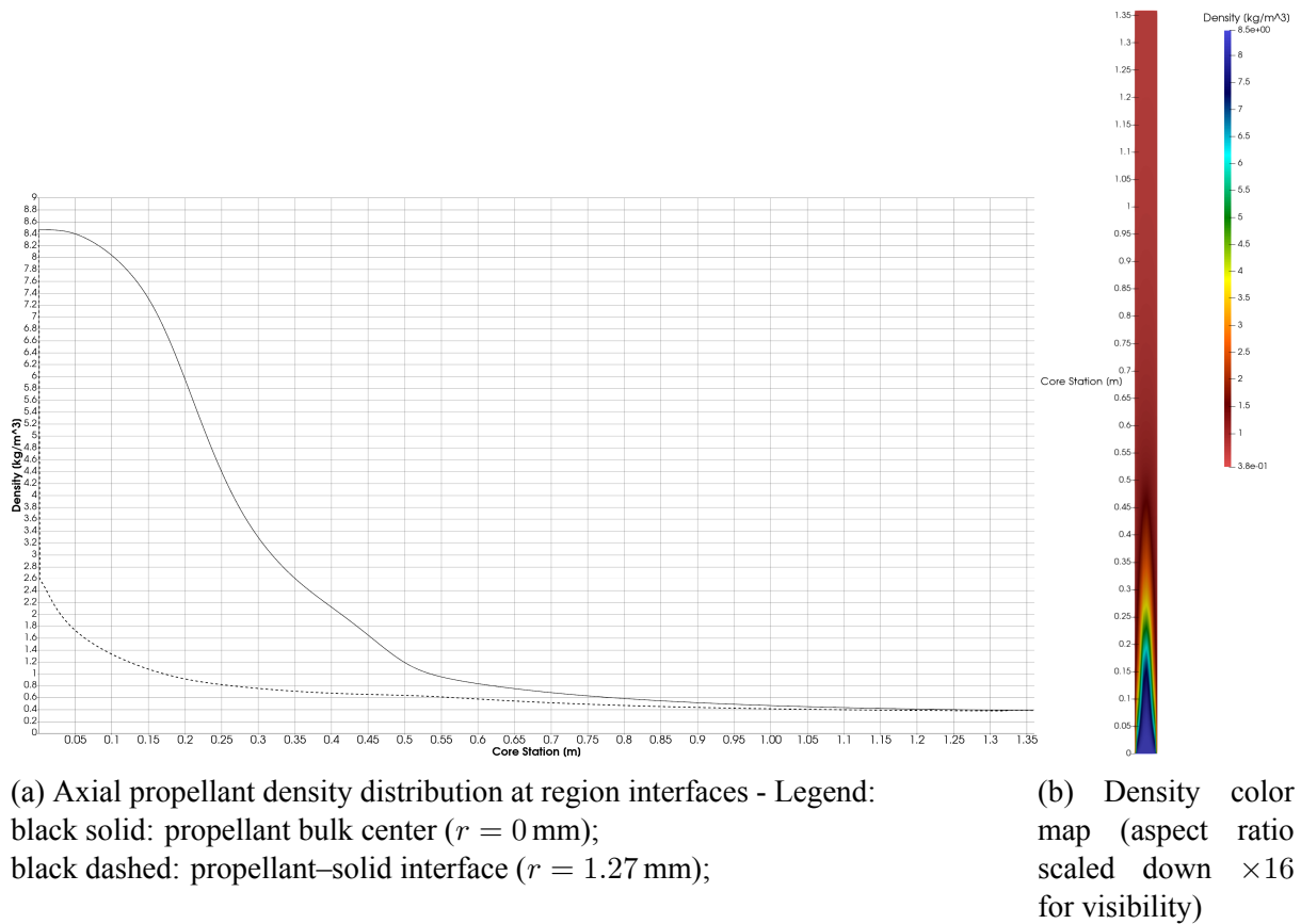
Figure 6.5: Axial graph and color map of diametral cut
