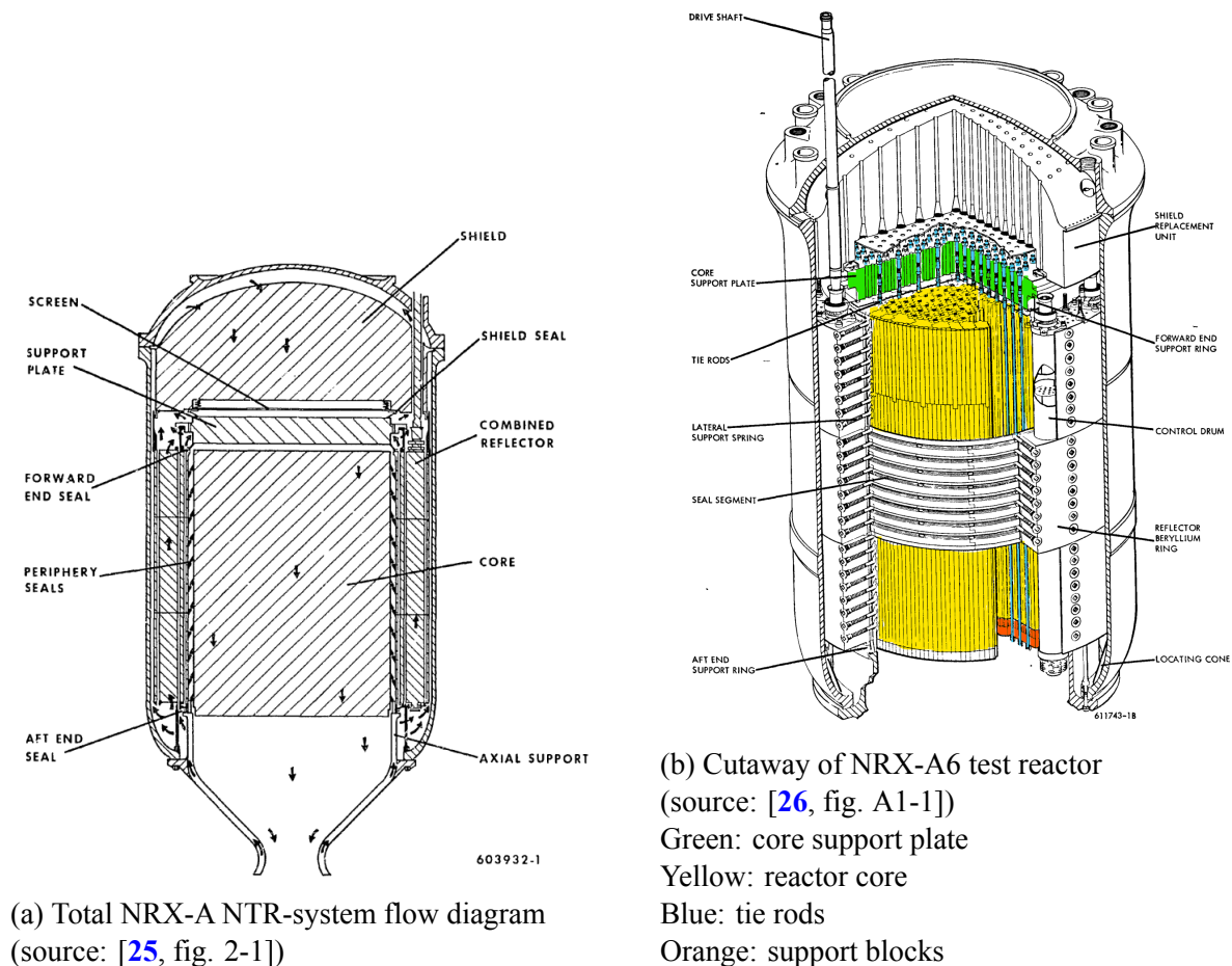
Figure 4.1: Flow schematic (a) and reactor cutaway
