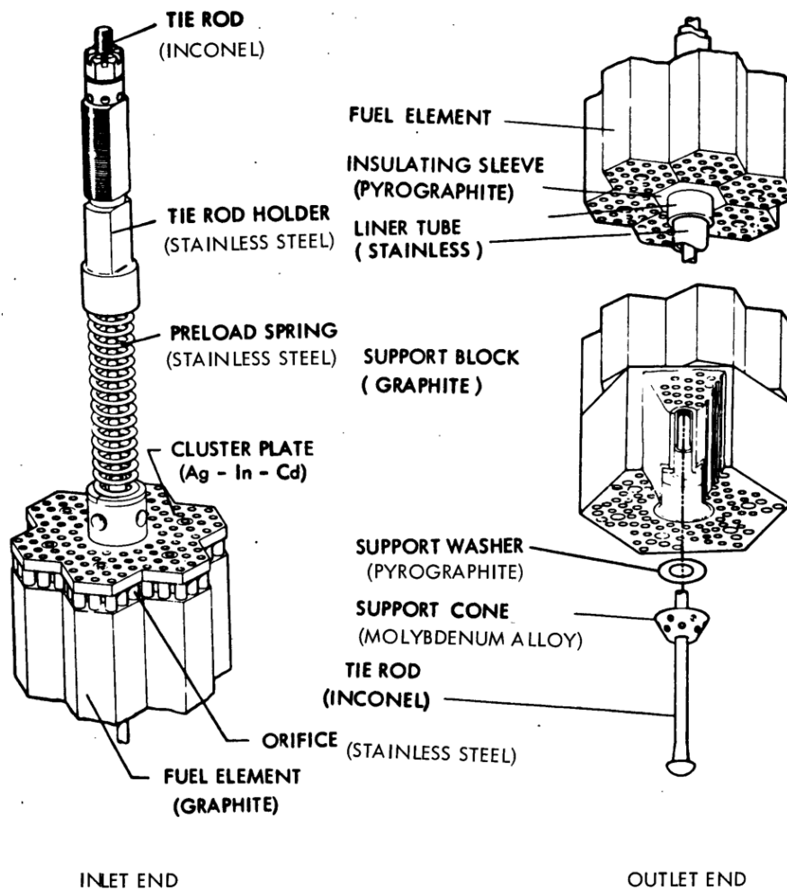
FIGURE 3-3 REGULAR FUEL CLUSTER
