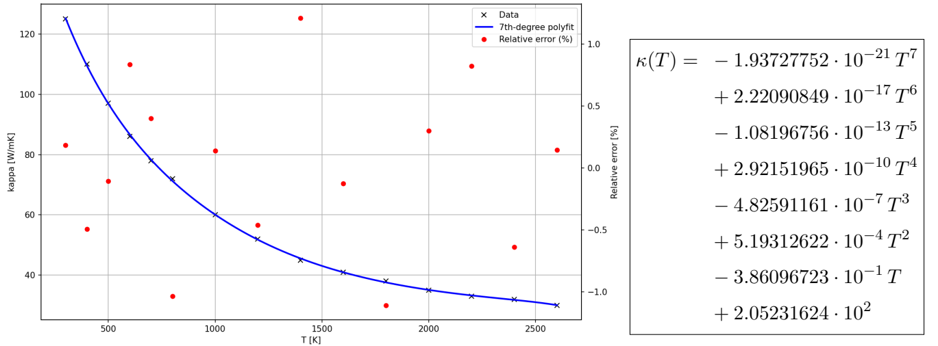
Figure 5.8: Polynomial fit for ATJ-S graphite thermal conductivity, with relative error at the data points
