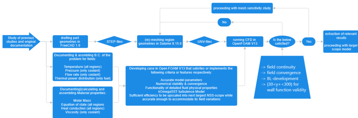
Figure 2.1: Workflow for CFD Model Development
