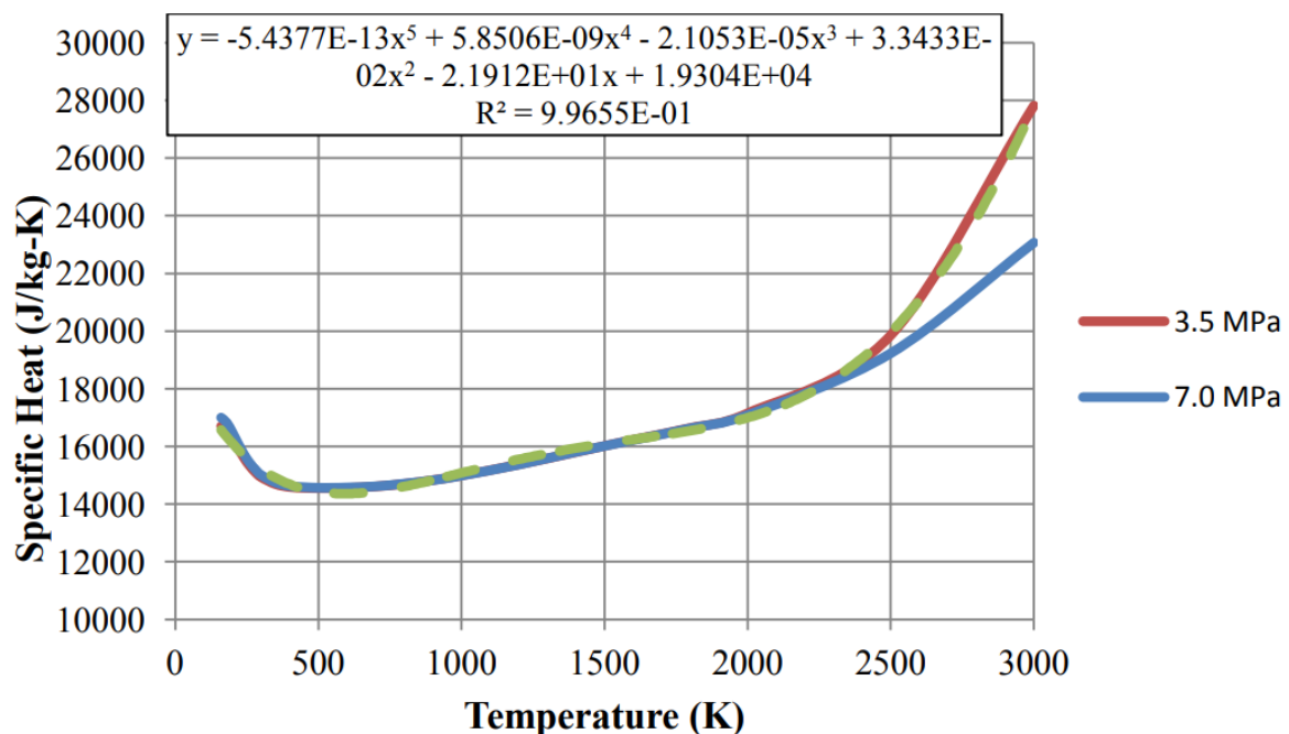
Figure A.1: Polynomial fit for specific heat c_p of hydrogen - Source: Brad Appel
